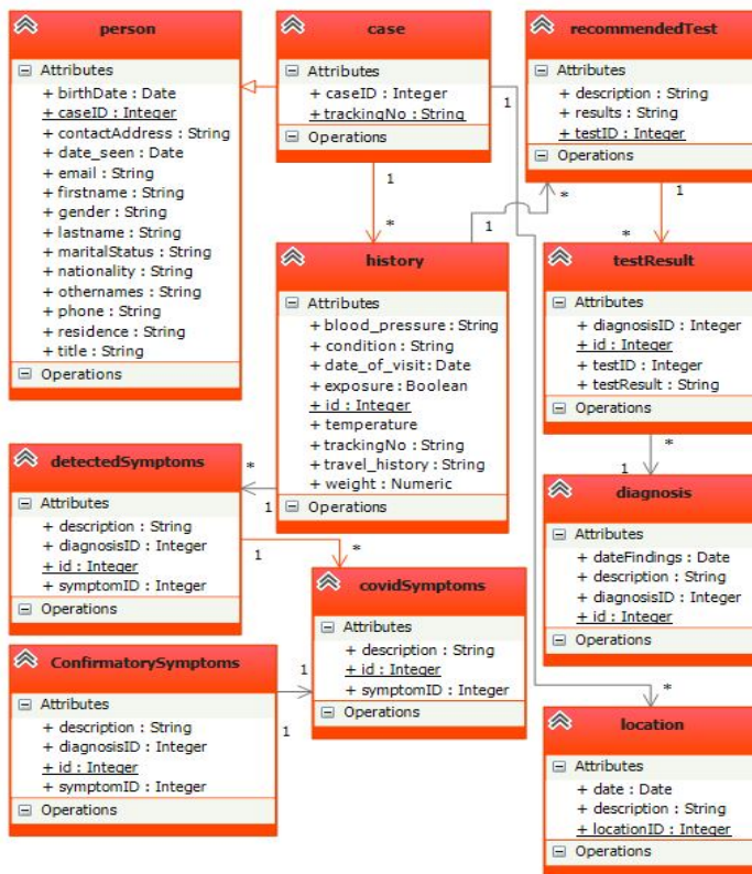
Figure 4: Low-level structure of the system using class diagrams
