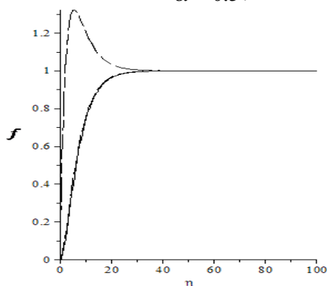
Figure 5: Graph of the velocity function f for various value of porous radial flow with constant viscosity when \alpha = 0.5 .
