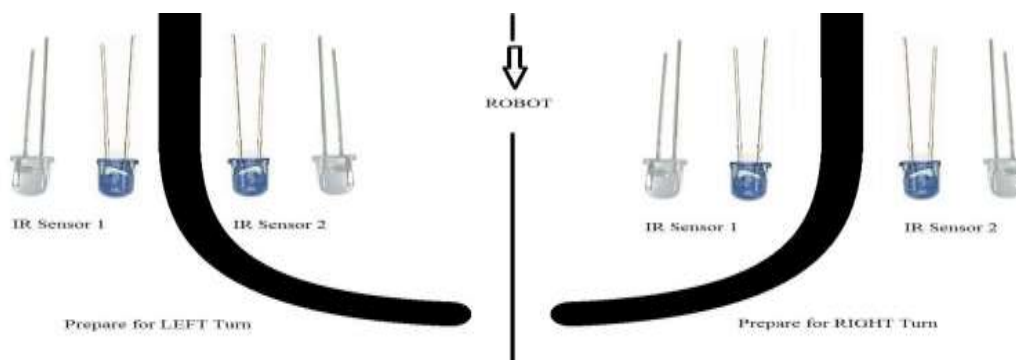
Figure 7: Left and Right turn configuration
