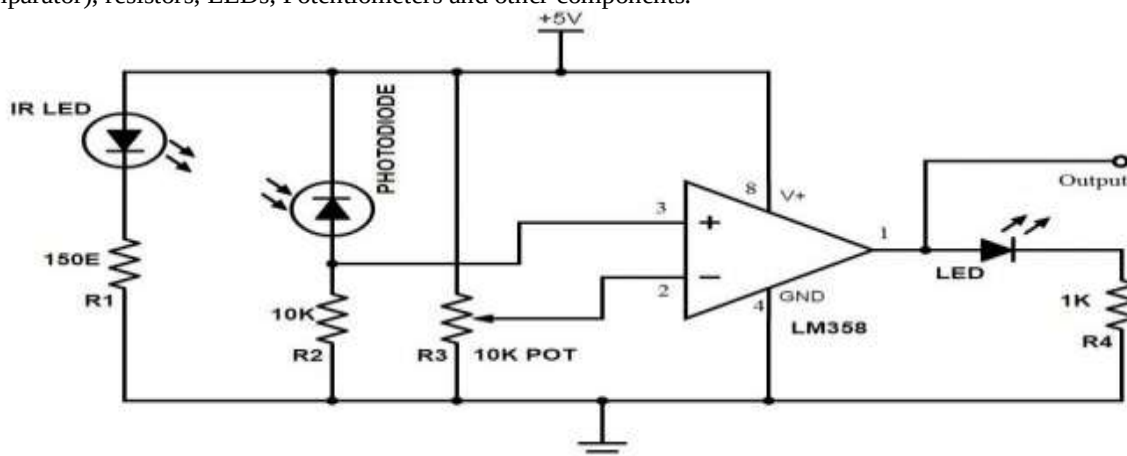
Figure 4: IR Sensor module design
