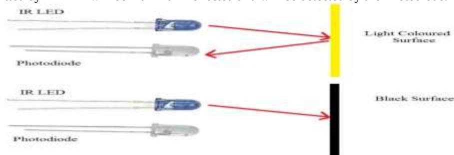
Figure 5: The working of a typical IR Sensor
