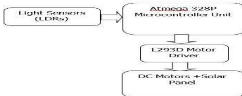
Figure 8: Solar tracking system model
