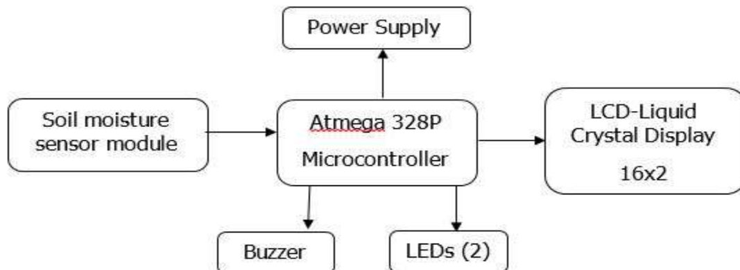
Figure 2: Soil moisture monitoring system
