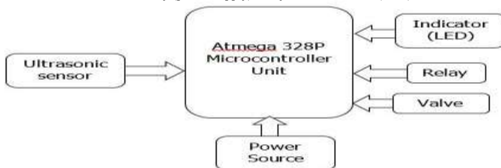
Figure 9: Refilling system model
