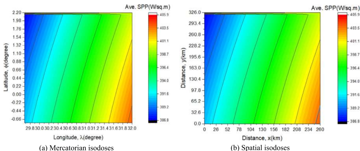
Fig. 7. (a, b) Mercatorian and spatial distribution of solar power potential for Western Region.
