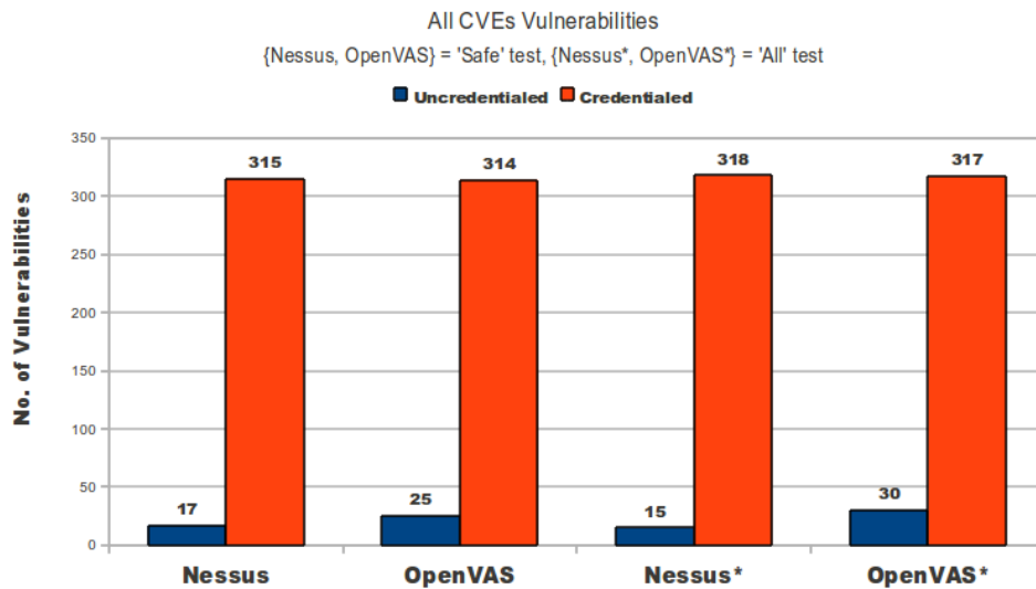
Figure 5. Nessus Vs. OpenVAS (All CVEs) Vulnerabilities
