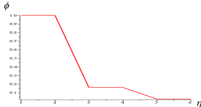
Figure 1: Graph of the temperature function g against the similarity variable \eta c = 0.4, b = 1.6
